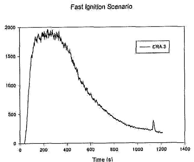
Figure A-10. HRR, Fast Ignition, Compartment Test
