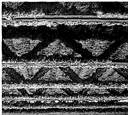
Figure C-4: Fireproofing added to structural steel
