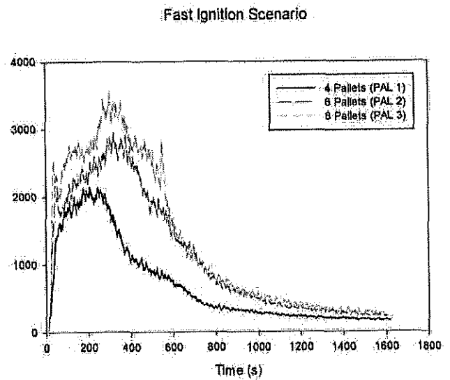
Figure A-8. HRR, Fast Ignition, Free Burn Scenario
