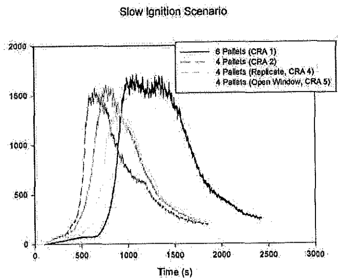
Figure A-9. HRR, Slow Ignition, Compartment Test
