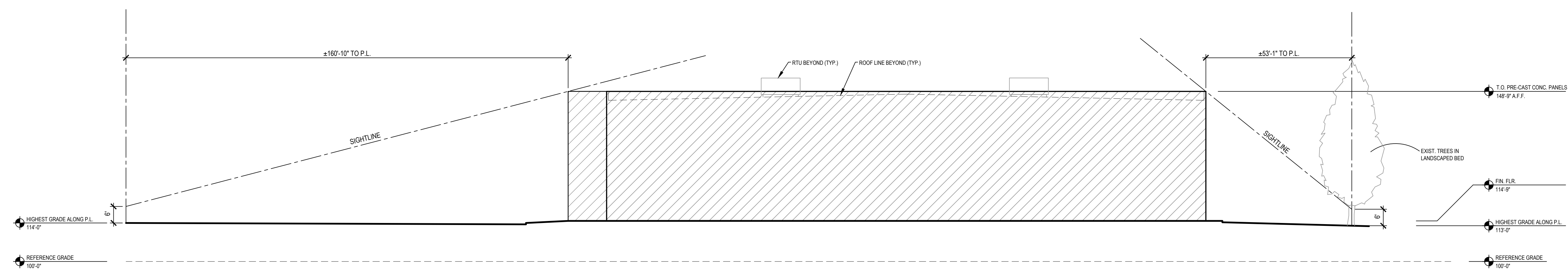
2 SIGHTLINE STUDY LONGITUDINAL VIEW SCALE: 1" = 20'-0"
