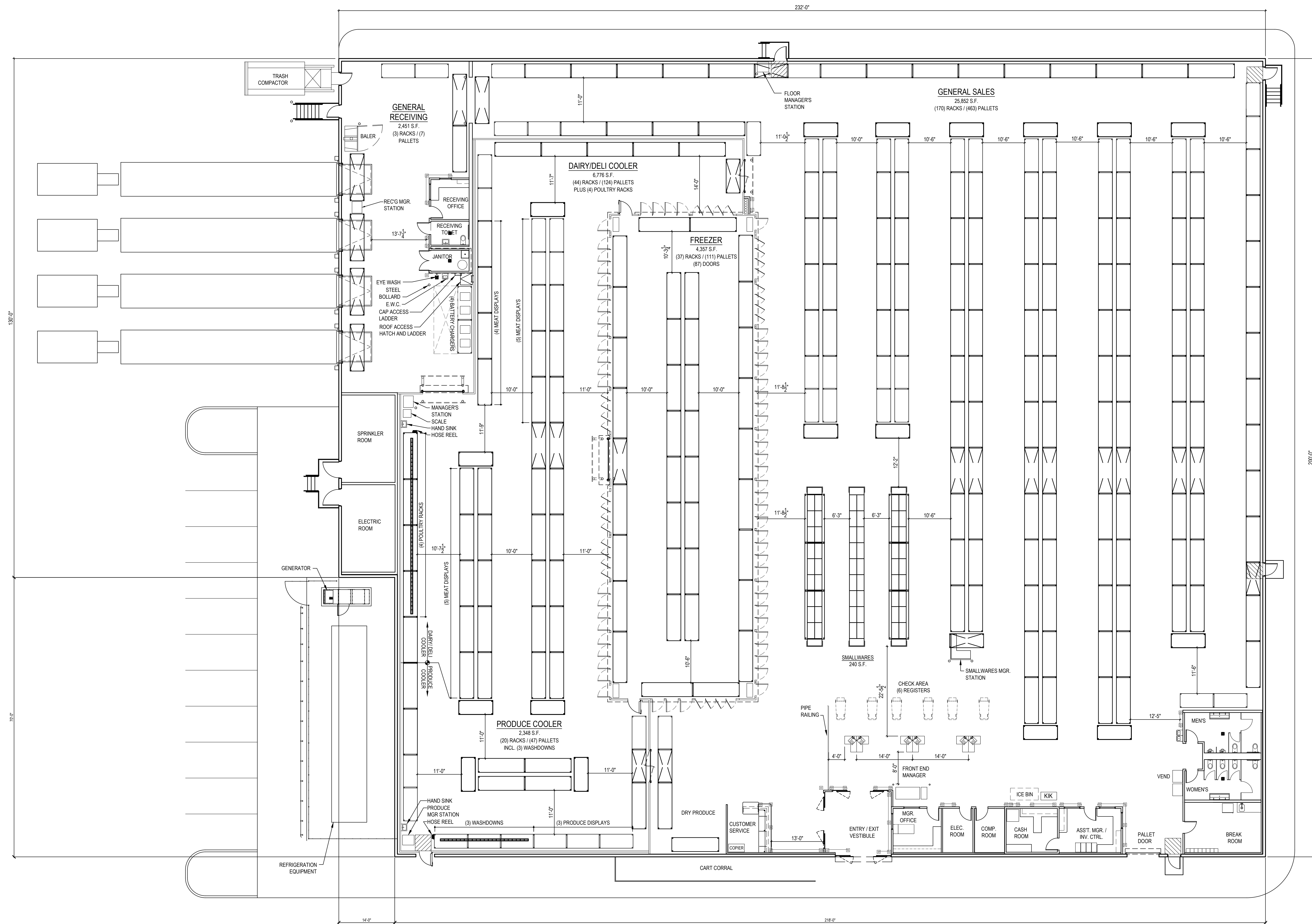
FIXTURE PLAN SCALE: 3/32"=1'-0"
