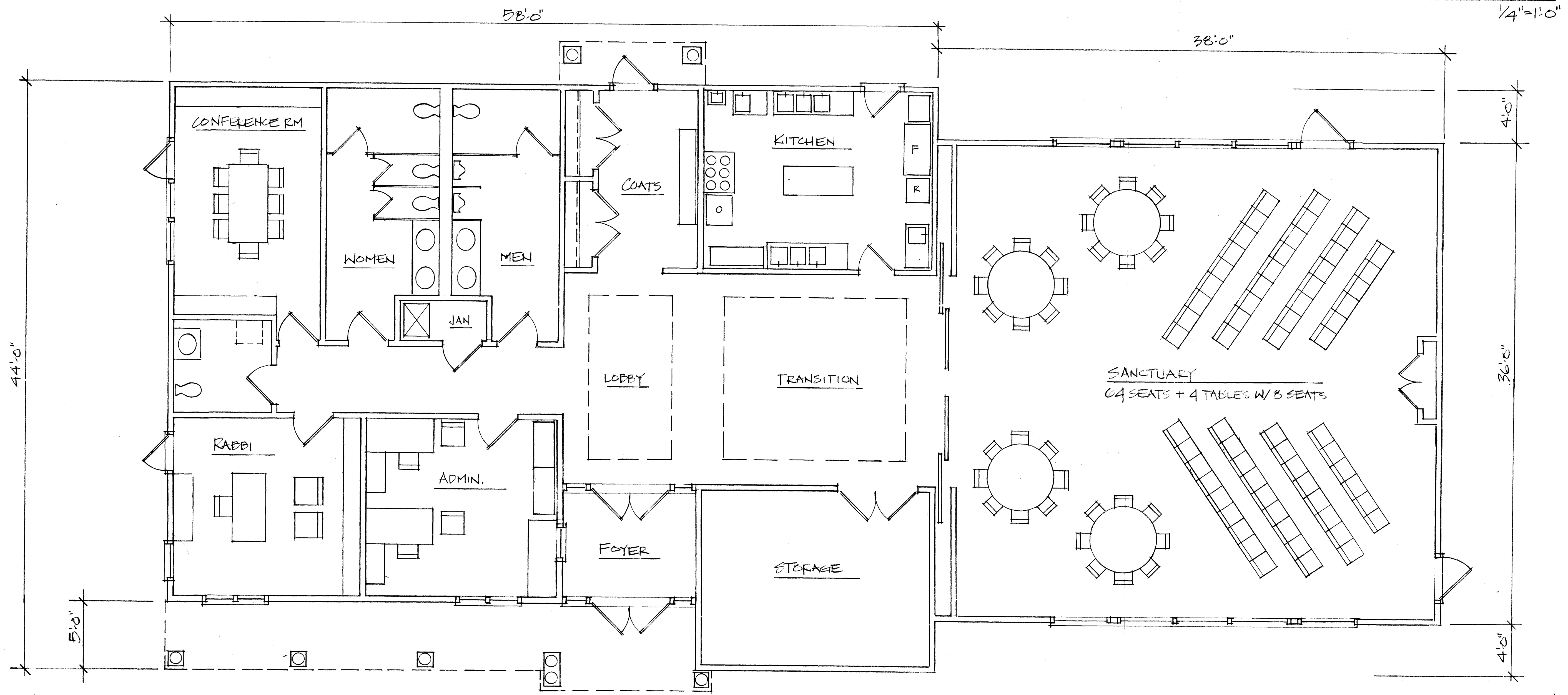
FLOOR PLAN - PROPOSED CONGREGATION BETH-EL - 33 KENYON ROAD - WATERFORD, CT
