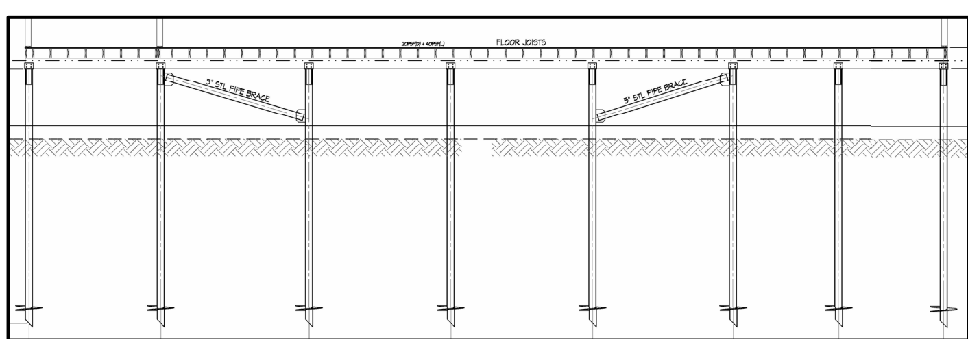
TYPICAL HELICAL PILE INSTALLATION
