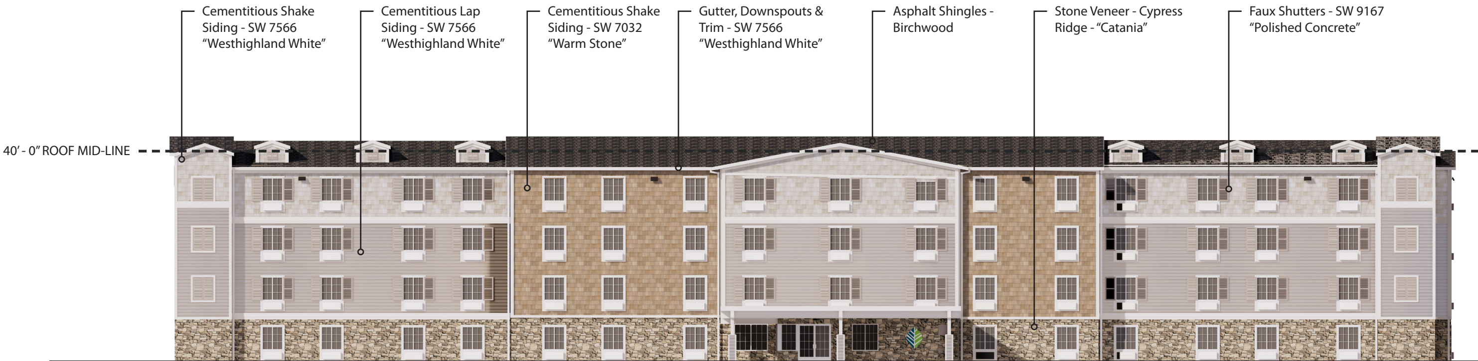
Front Elevation
