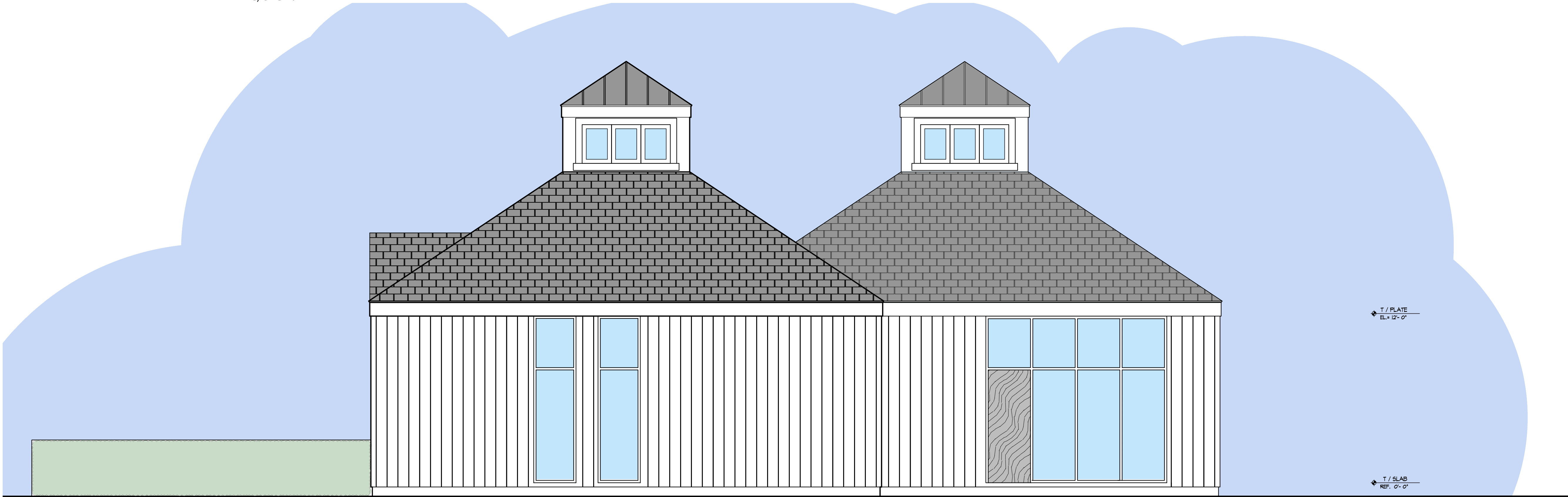
NORTH ELEVATION
