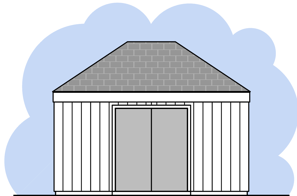
SOUTH ELEVATION 1/4"=1'-0"
