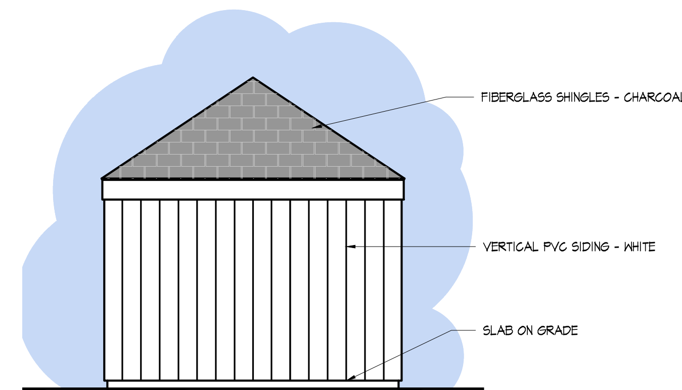
WEST ELEVATION 1/4"=1'-0"
