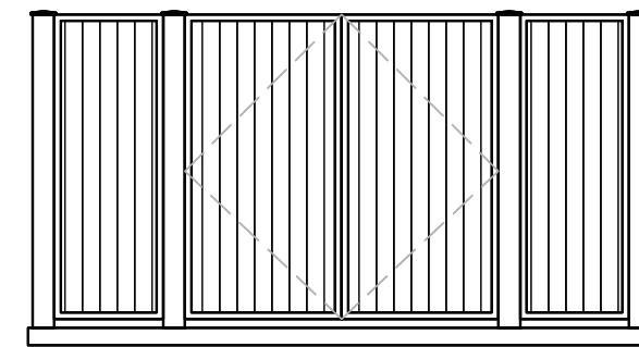
SOUTH ELEVATION 1/4"=1'-0"
