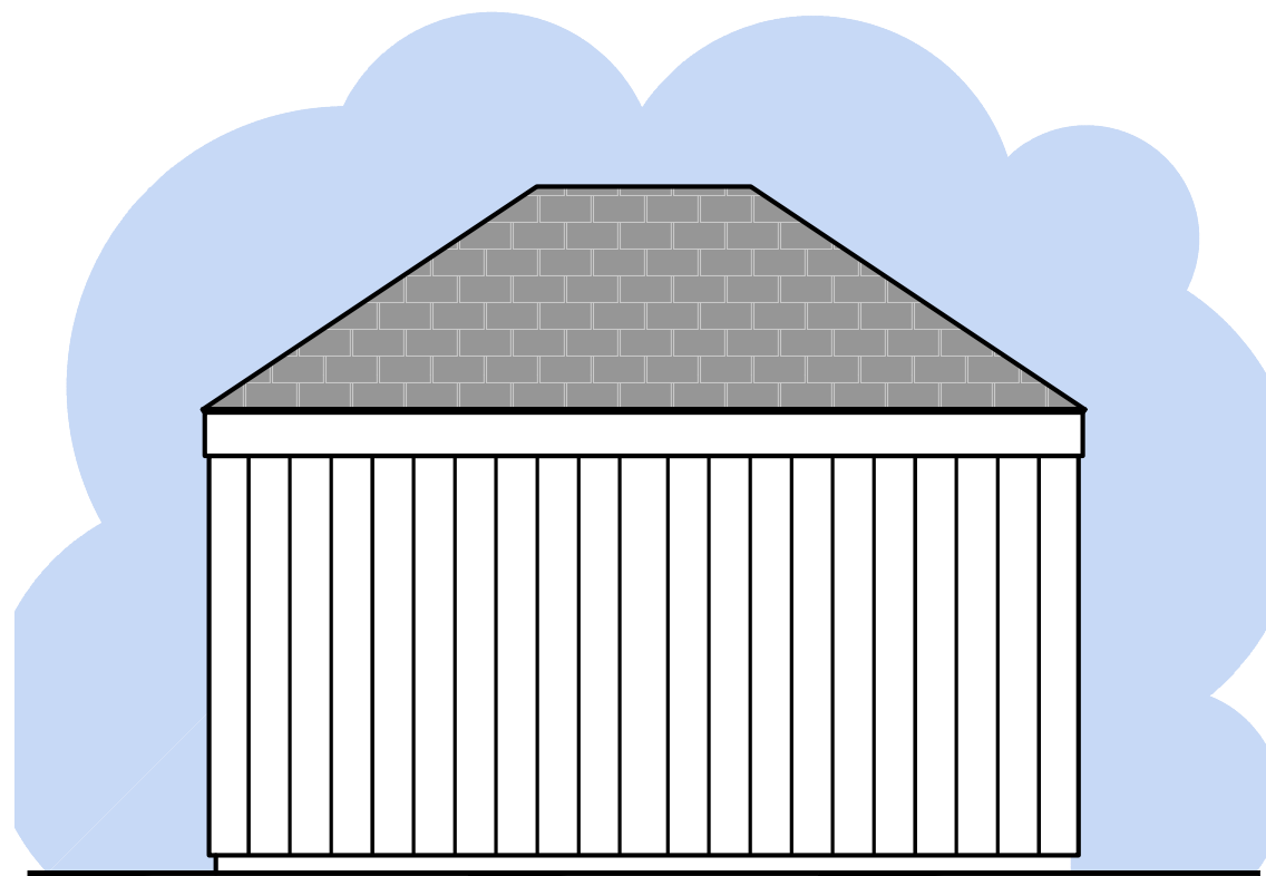
NORTH ELEVATION 1/4"=1'-0"
