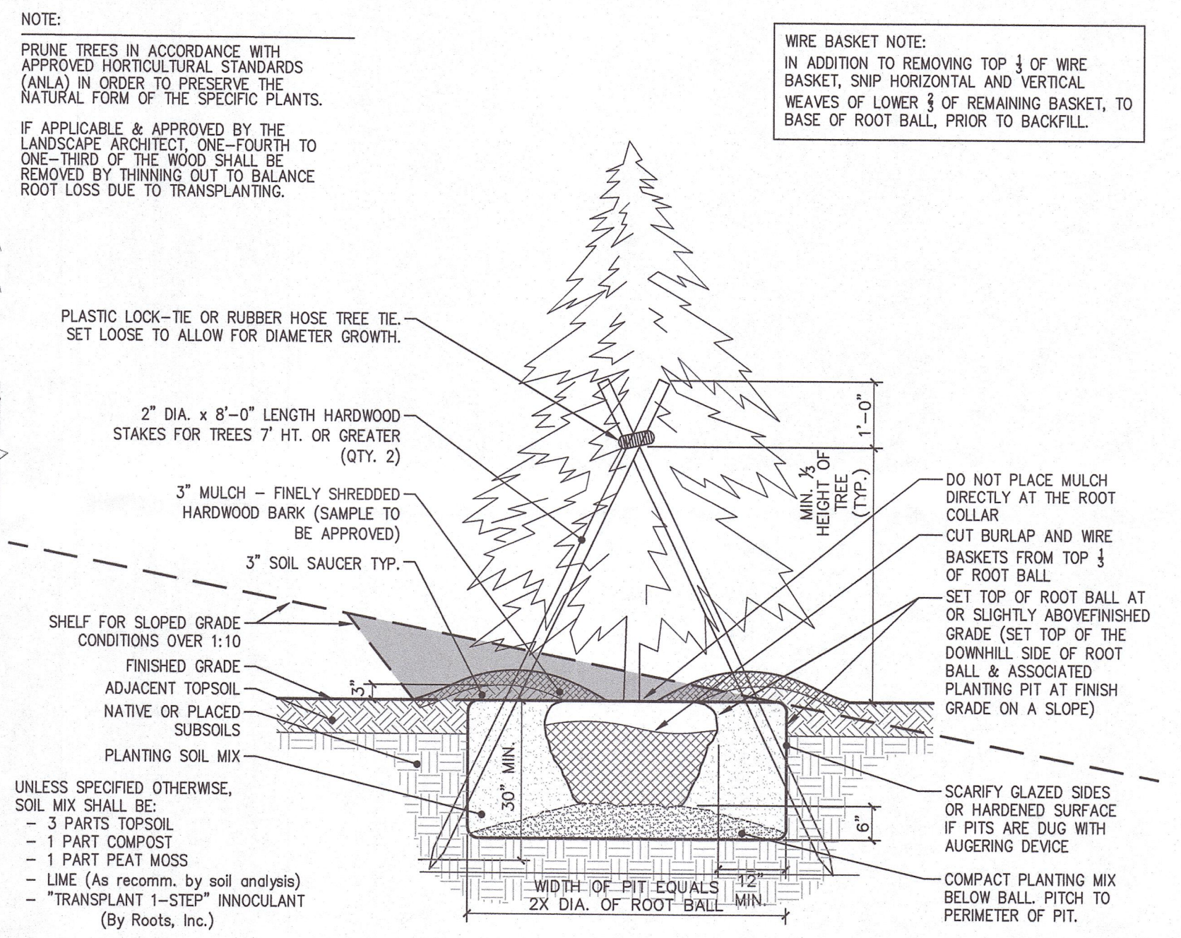
2 CONIFER TREE PLANTING DETAIL SCALE: 1/2" = 1'-0"
